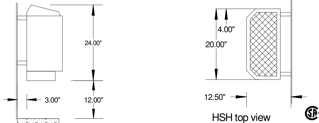
HSH side view
