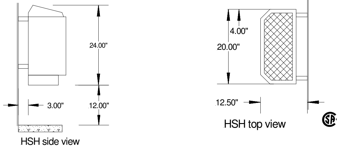
Heater Location
